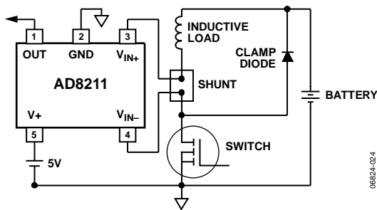
Figure 25. Low-Side Switch
