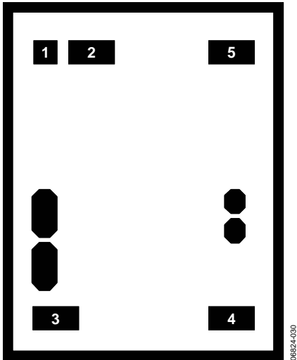
Figure 2. Metallization Diagram
