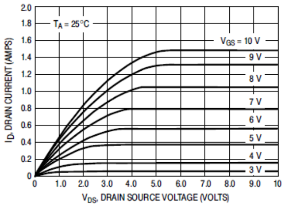
Figure 3. Ohmic Region
