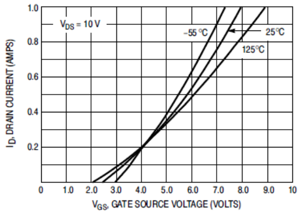
Figure 4. Transfer Characteristics
