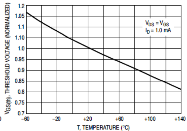
Figure 6. Temperature versus Gate Threshold Voltage
