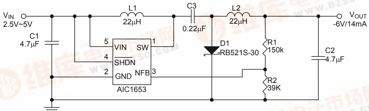
L1,L2: TOKO D312F 22 \mu H D1: Rohm RB521S-30 C1,C2,C3: TAIYO YUDEN Ceramic capacitors
