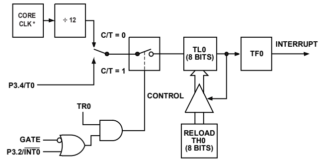
Figure 77. Timer/Counter 0, Mode 2
