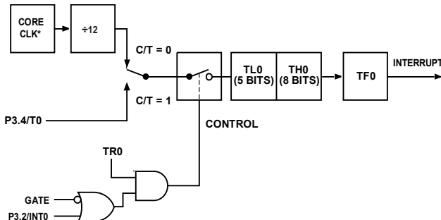
Figure 75. Timer/Counter 0, Mode 0
