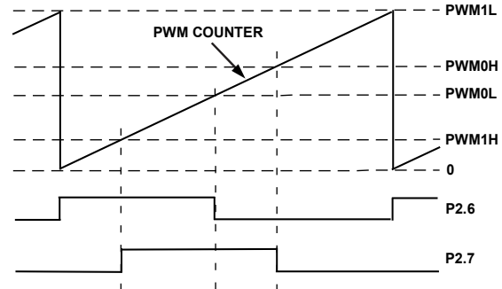
Figure 58. PWM Mode 2
