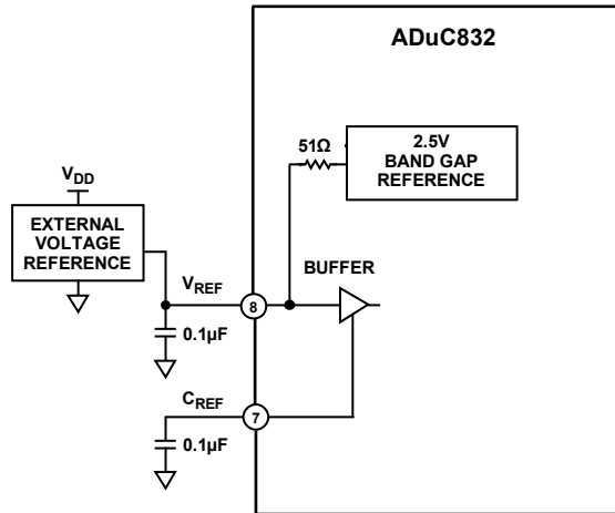
Figure 43. Using an External Voltage Reference
