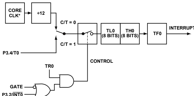
Figure 76. Timer/Counter 0, Mode 1
