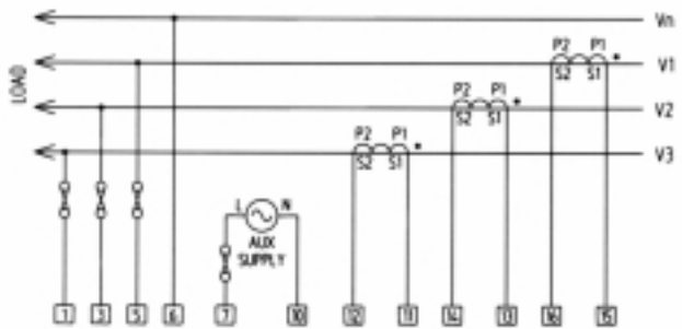
3-Phase 4-Wire
