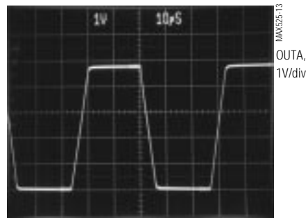
DYNAMIC RESPONSE
