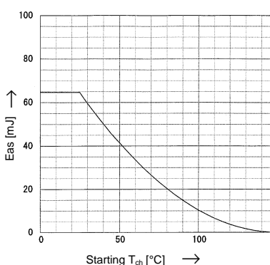
Avalanche Energy Derating E_{as} = f(\text{starting } T_{ch}) ; V_{CC} = 60\text{V} ; I_{AV} = 10\text{A}
