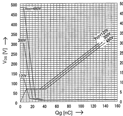
Typical Gate Charge Characteristic V_{GS} = f(Q_g) ; I_D = 10\text{A} ; T_{ch} = 25^\circ\text{C}
