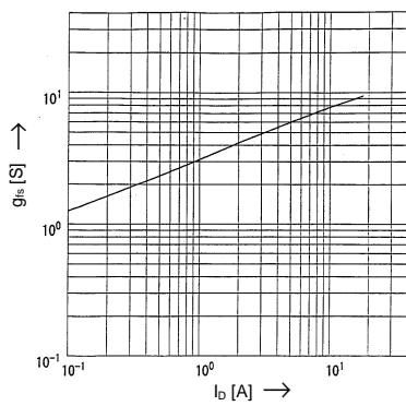
Typical Forward Transconductance vs. I_D g_{fs} = f(I_D) ; 80μs pulse test; V_{DS} = 25\text{V} ; T_{ch} = 25^\circ\text{C}
