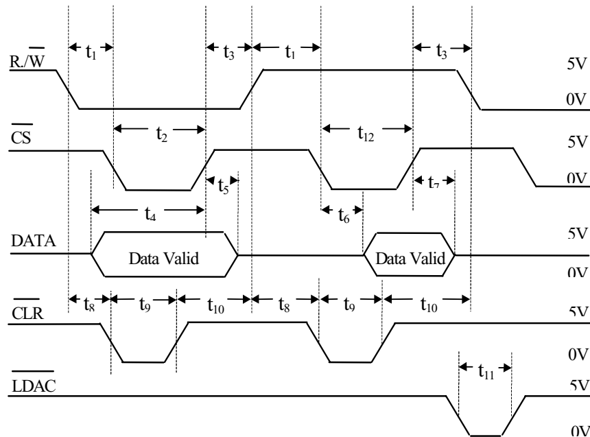
FIGURE 3. 16-BIT DIGITAL TO ANALOG CONVERTER
