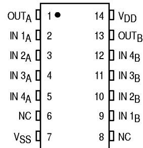
MC14082B Dual 4-Input AND Gate
