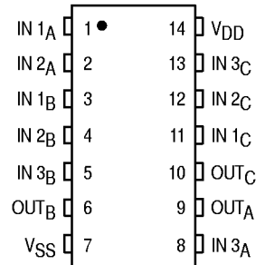
MC14075B Triple 3-Input OR Gate
