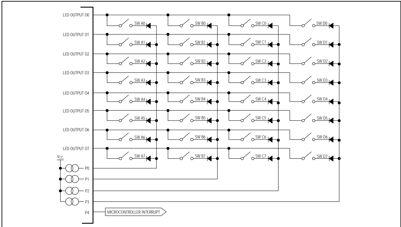
Figure 7. Key-Scanning Configuration
