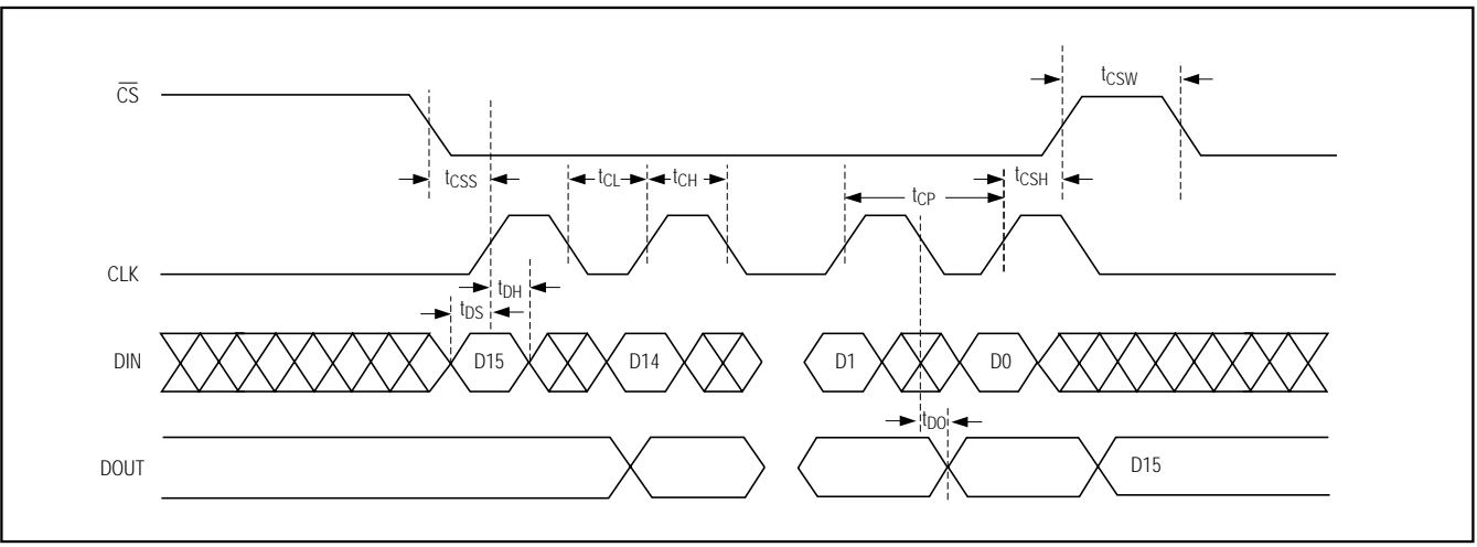
Figure 3. Timing Diagram
