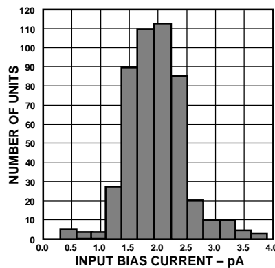
Figure 5. Typical Distribution of Input Bias Current (570 Units)
