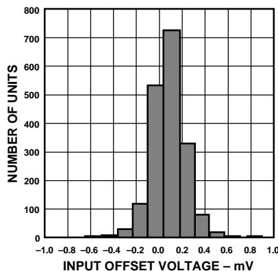
Figure 4. Typical Distribution of Input Offset Voltage (1055 Units)
