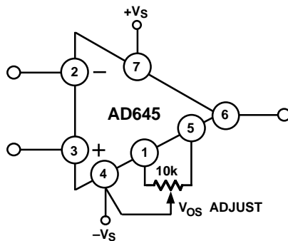
Figure 3. AD645 Offset Null Configuration
