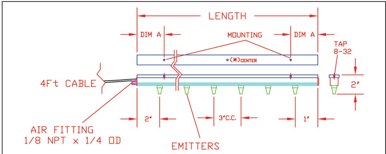
Figure 2. SPI Air-Assisted Ion Bar dimensions
