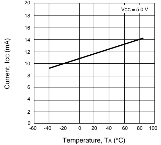
UPC2712TB CURRENT vs. TEMPERATURE
